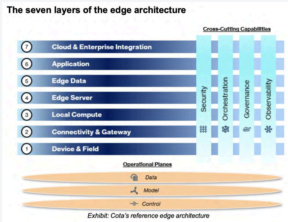
Figure 1: Cota's reference edge architecture
